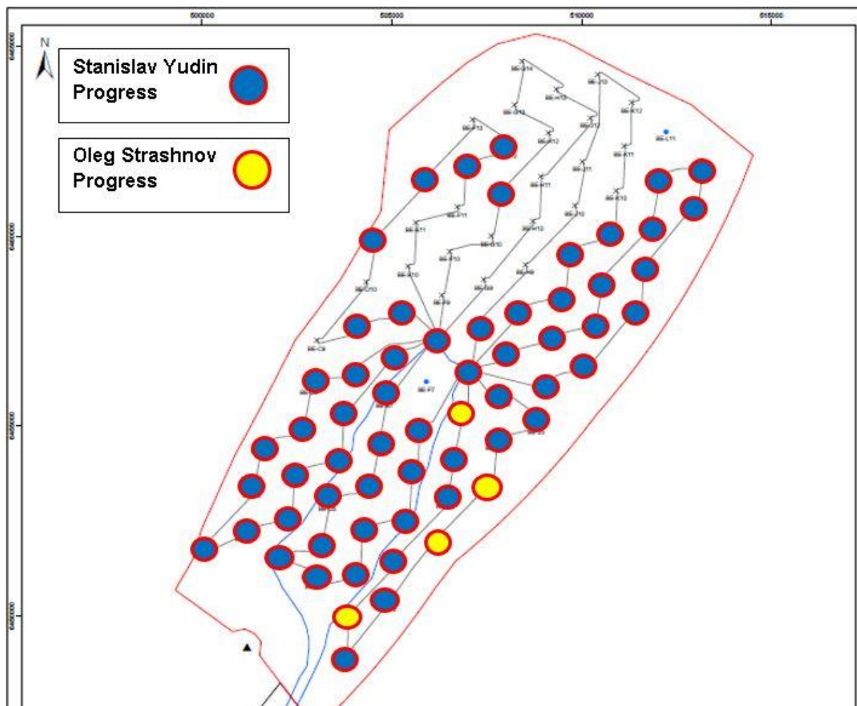
Fig 2 – Piled locations & Installed Jacket locations.
