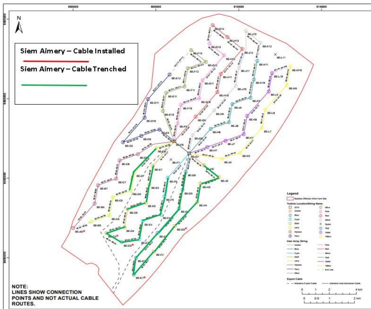
Fig. 7 Cable installation Progress
