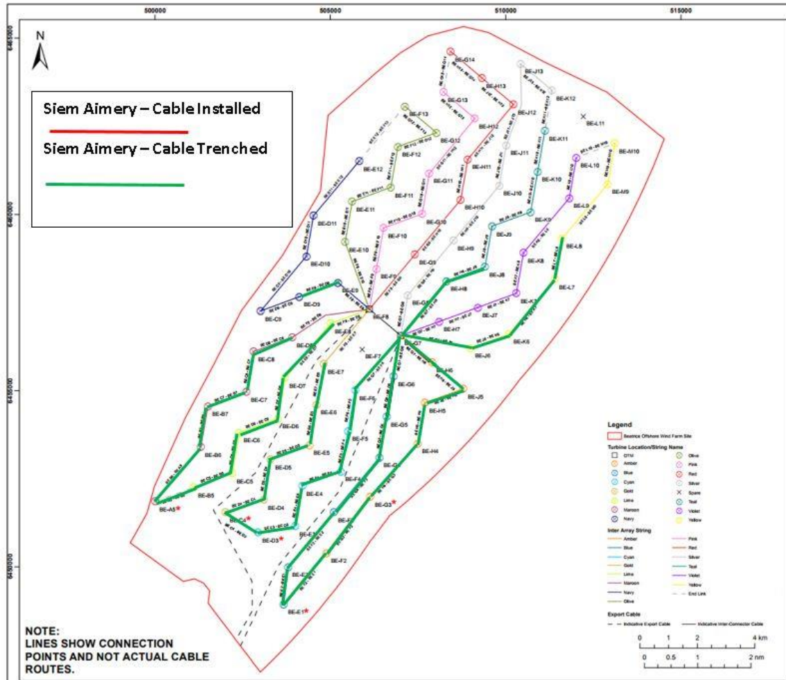
Fig. 3 Cable installation Progress
