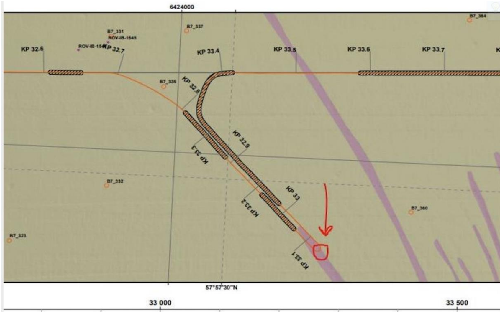
Fig 2. Location of exposed Cable on EC2
