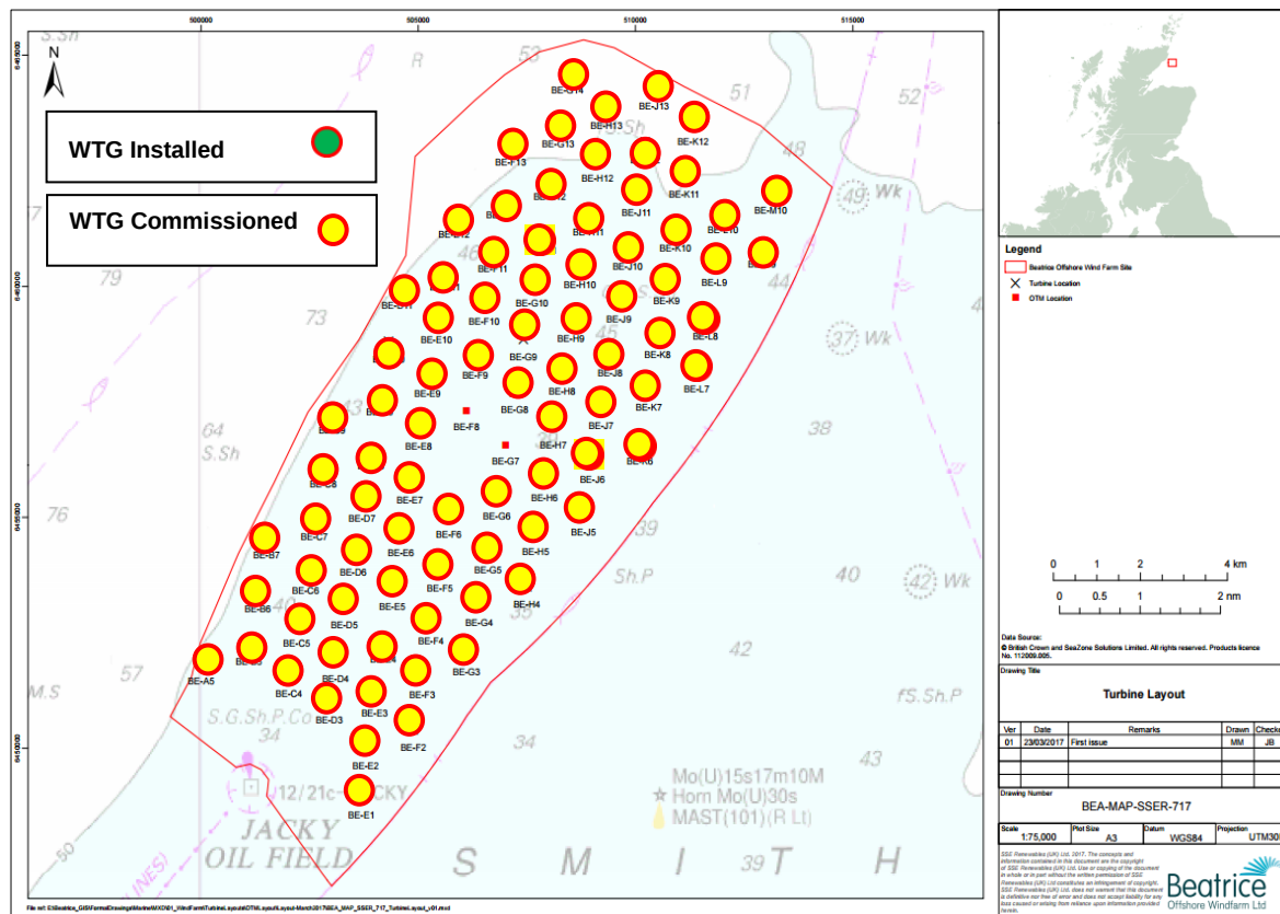
Fig. 2 Locations of WTG in the BOWL Construction Site
