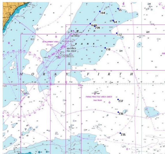
Fig. 6 Scientific equipment locations
